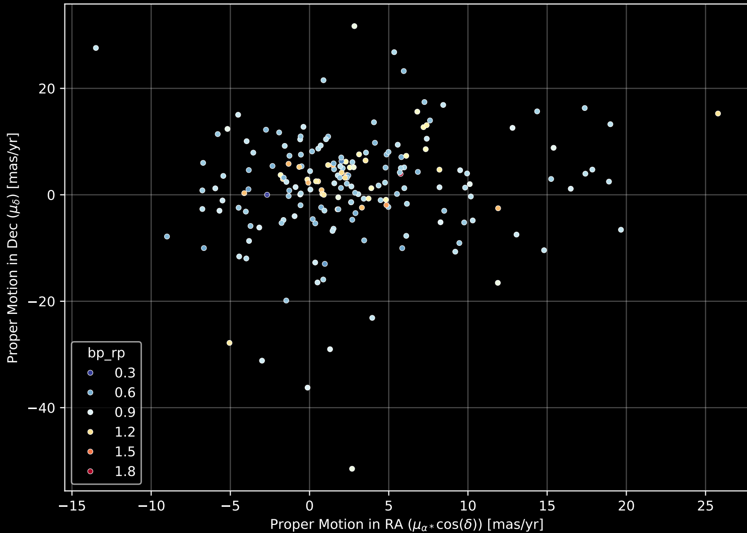
GALAH DR4 Field: [529] Proper Motion Diagram (n= 187)
