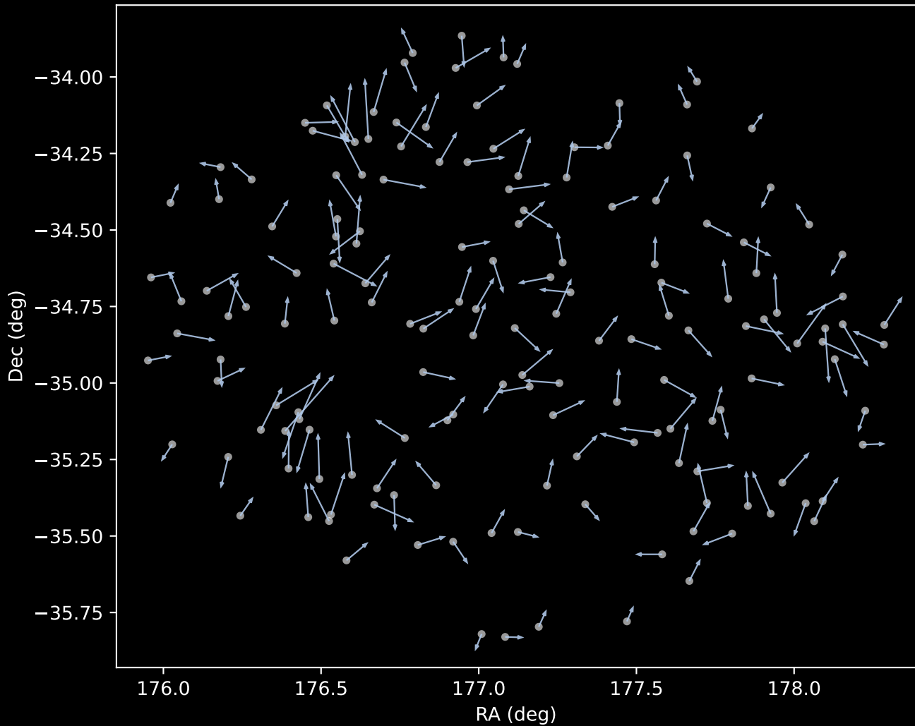
GALAH DR4 Cluster 1 Proper Motion Vectors (n=160)
