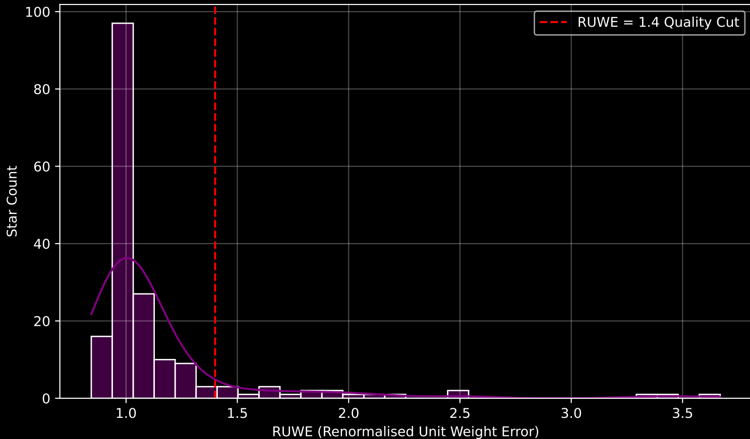
GALAH DR4 Field [529] RUWE Distribution (n= 182)
