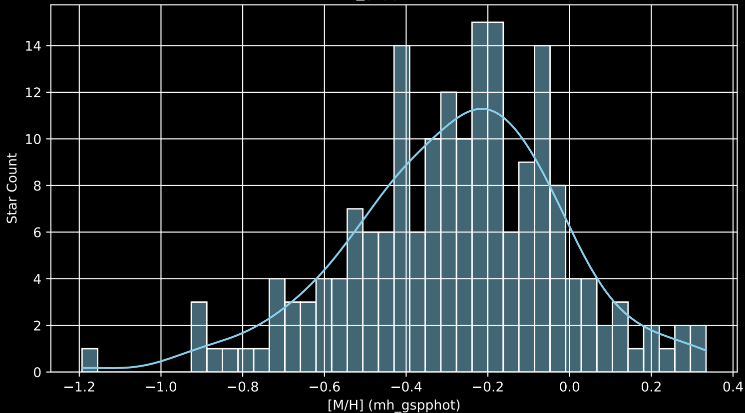
GALAH DR4 Field: [529] [M/H] (mh_gspphot) (n= 185)
