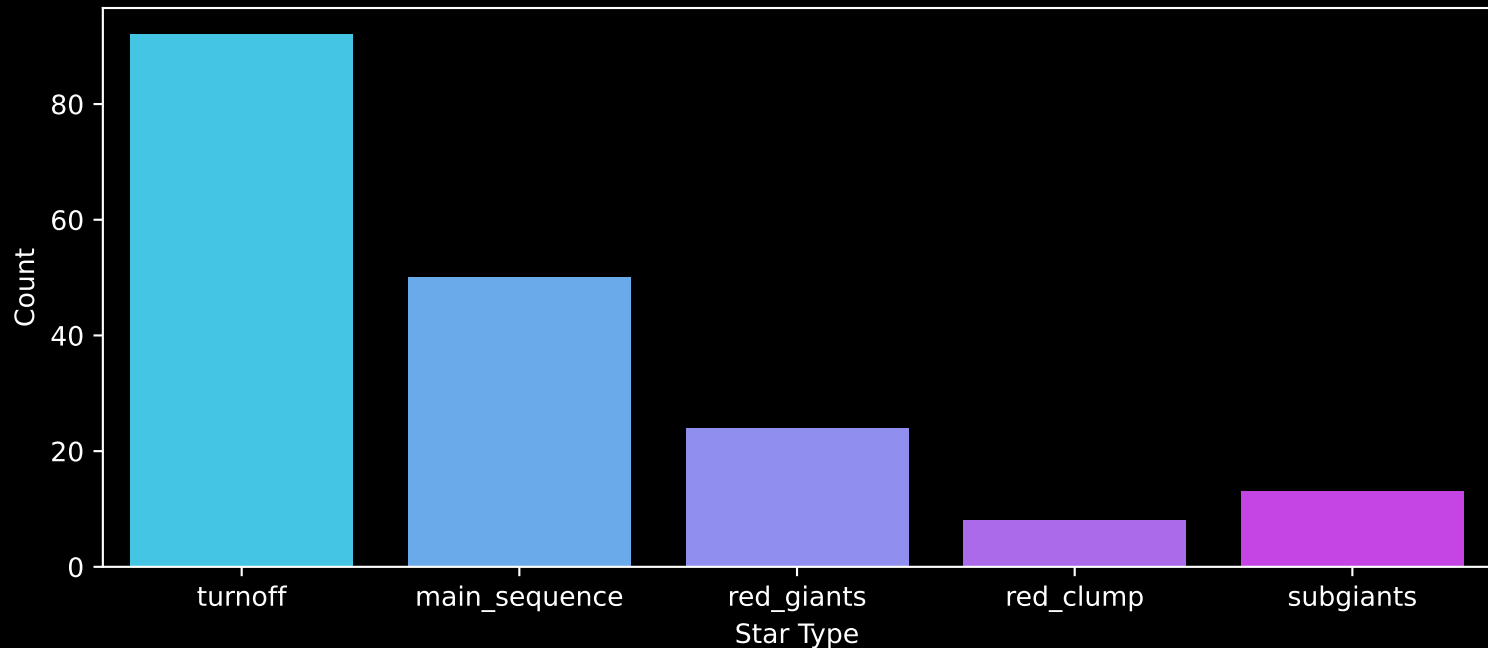
GALAH DR4 Field: [529] Count plot of Star Type
